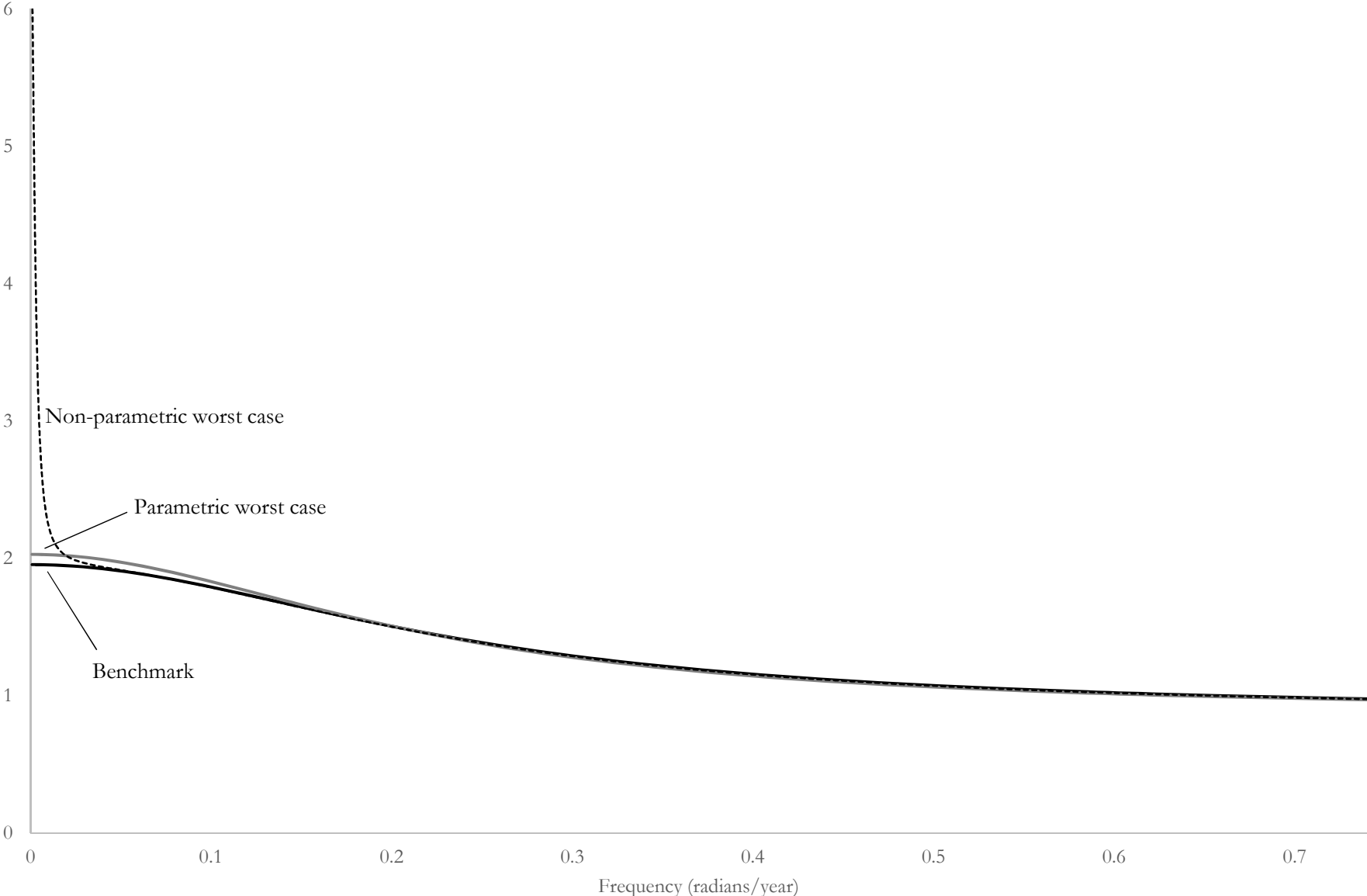
Figure 3. Benchmark and worst-case transfer function
